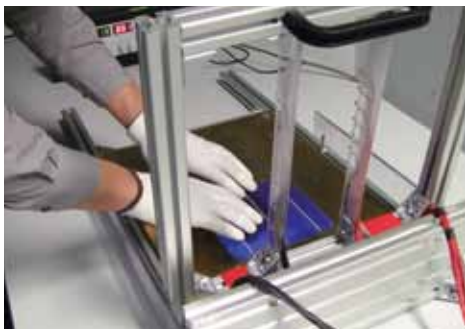
In the SOLON labs the cell is placed under reversed bias and inspected using a FLIR thermal imaging camera to detect shunts.
