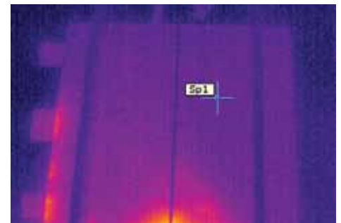
This thermal image shows that this cell has flaws in the edge isolation, which causes local shunts.
